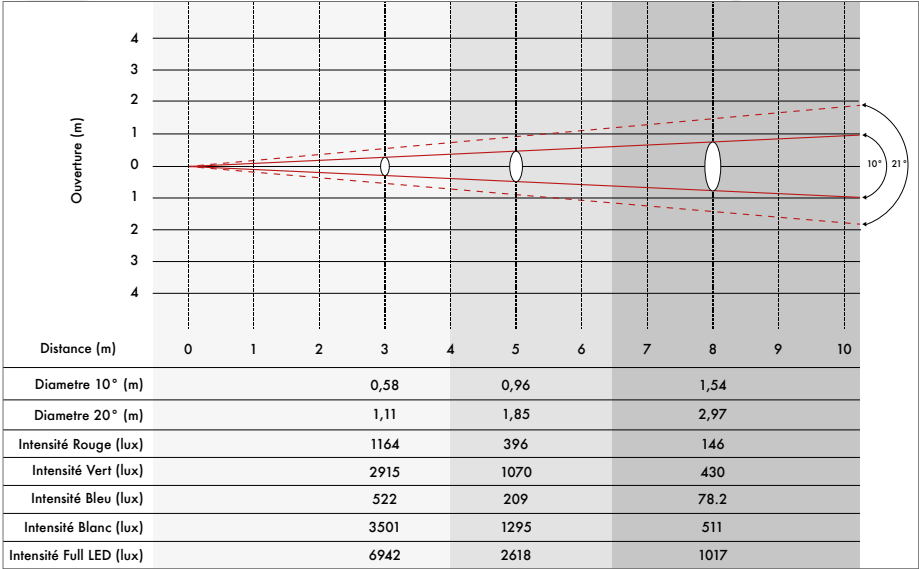
Angle beam 10° / Angle field 21°
