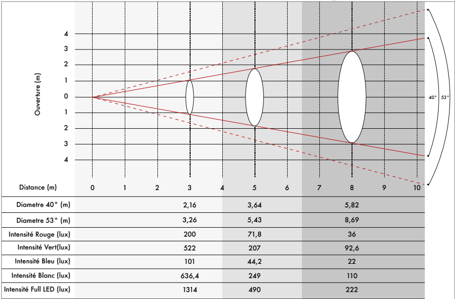
Angle beam 40° / Angle field 53°
