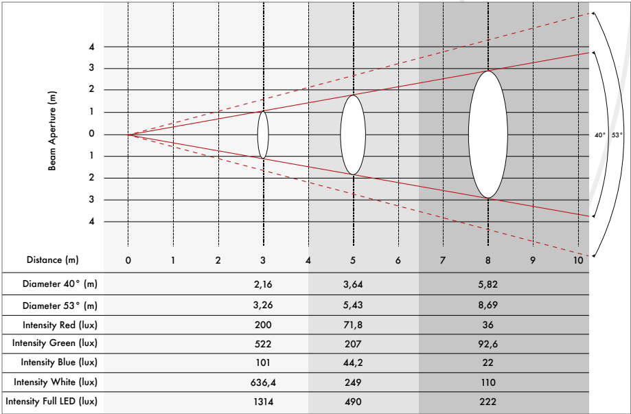
Beam angle 40° / Field angle 53°
