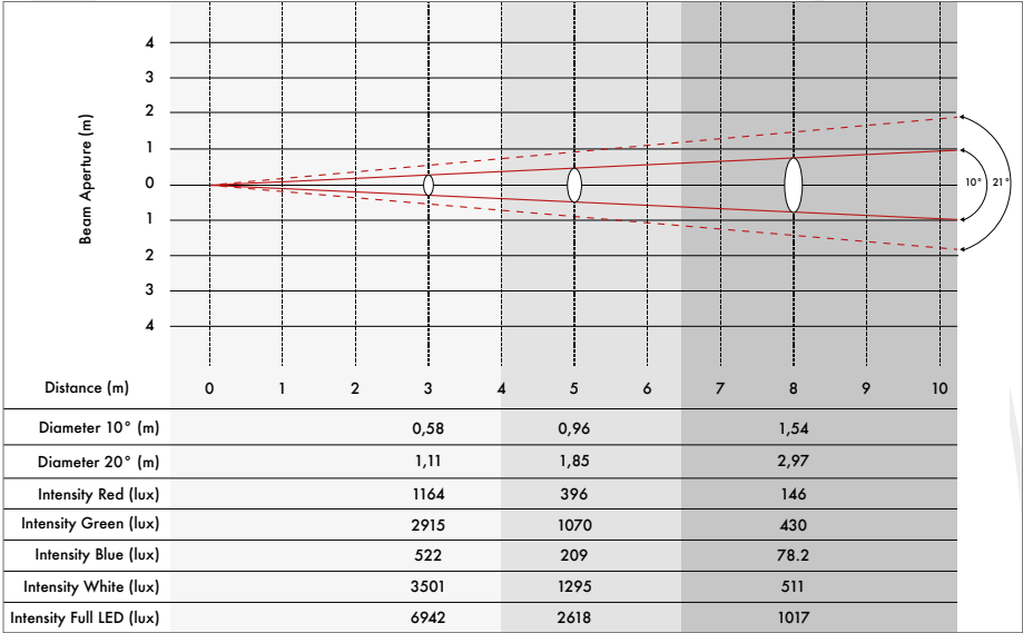
Beam angle 10° / Field angle 21°
