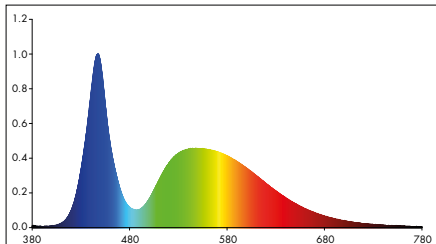
Full WHITE (wide beam) : Flux=3439 lm*
